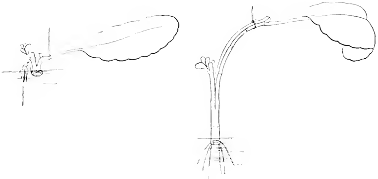
FIG. 86.—When the apical leaf is near the base of the stem (left), callus is formed more rapidly than when apical leaf is at greater distance from the base of stem. Nov. 30 to Dec. 14, 1923.
